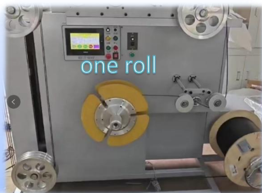
Fiber optic FTTH drop cable cutting machine 2.0*3.0mm indoor or 2.0*5.0mm outdoor cable /WTTX-600P
