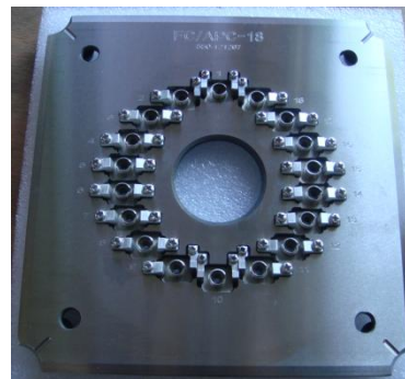
18 port
