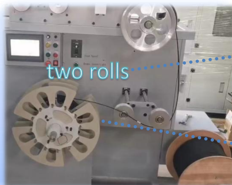
Fiber optic FTTH drop cable cutting machine 2.0*3.0mm indoor or 2.0*5.0mm outdoor cable /WTTX-600P
